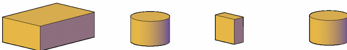
Original Objects
