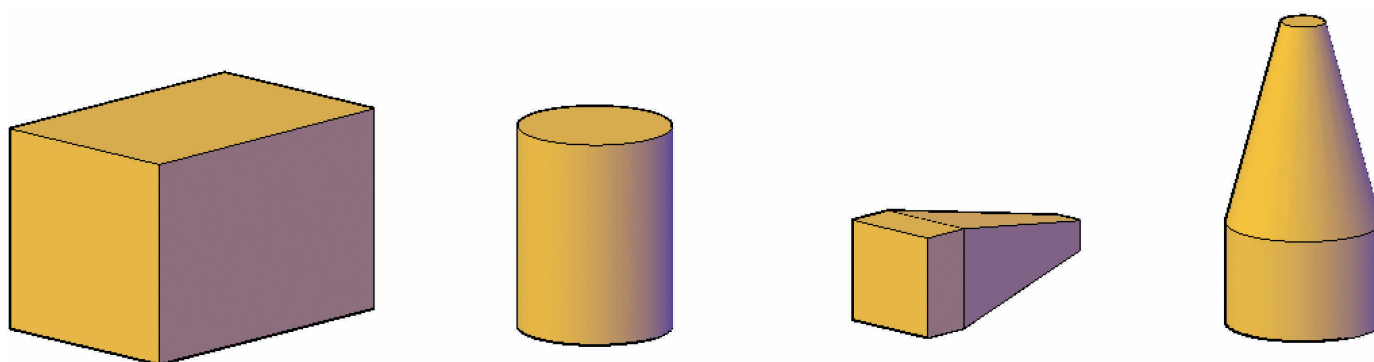
Modified Objects
