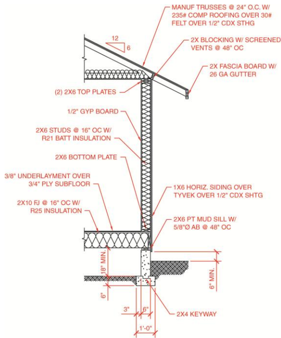
Wall Section
