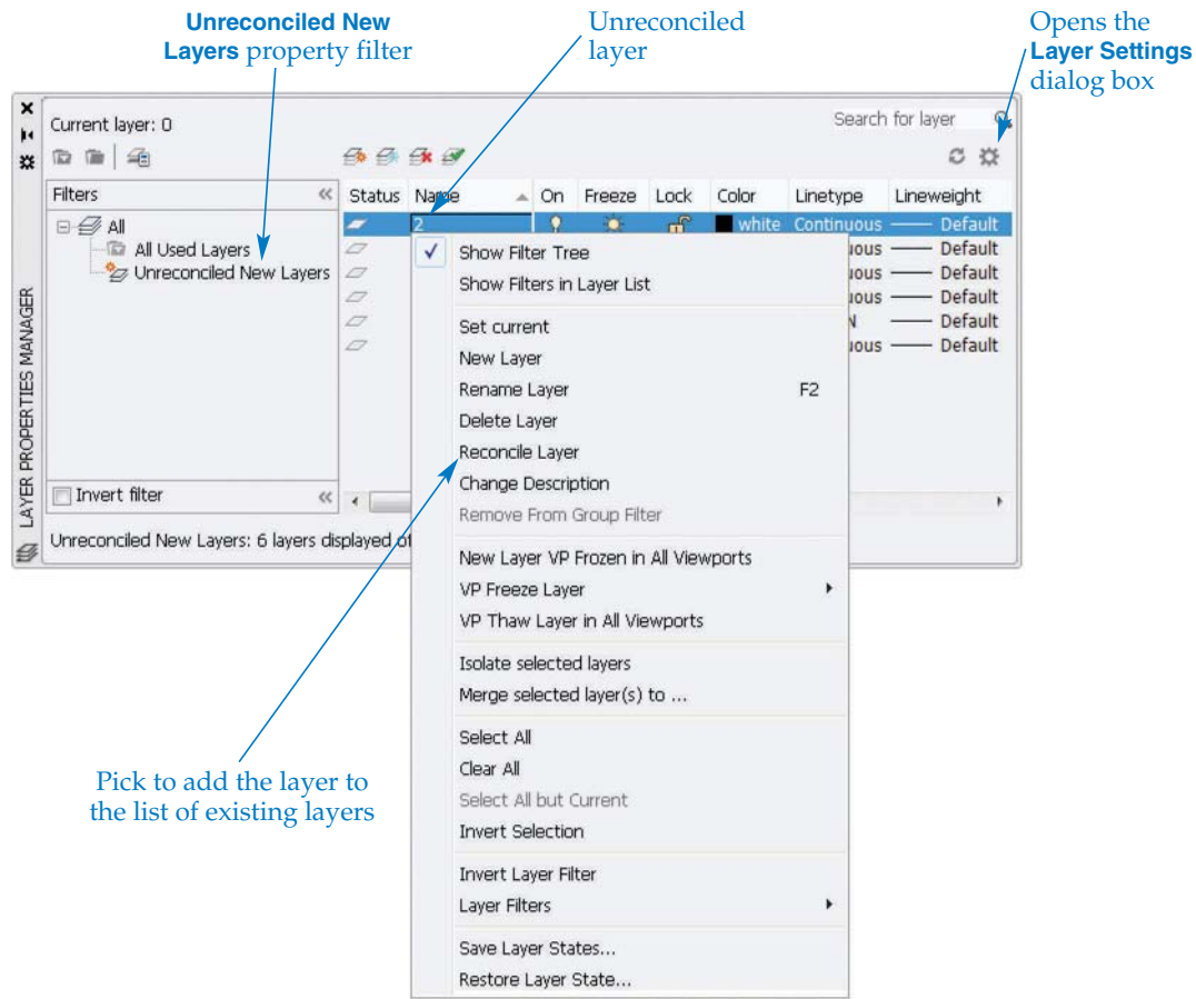
Figure 5C-2. Reconciling a new layer.
