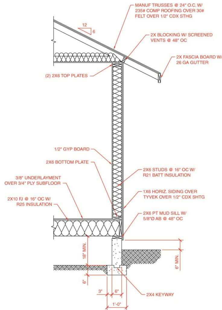
Wall Section A
